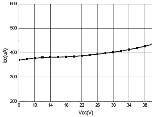
Figure 1. Operating Current Vs. Vcc Voltage
